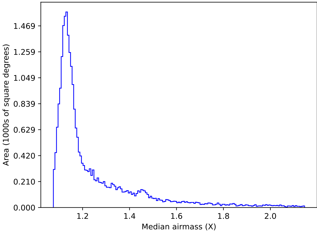
too_elab_r8_d2_gz_v3.4_10yrs All sky r band: Median airmass
