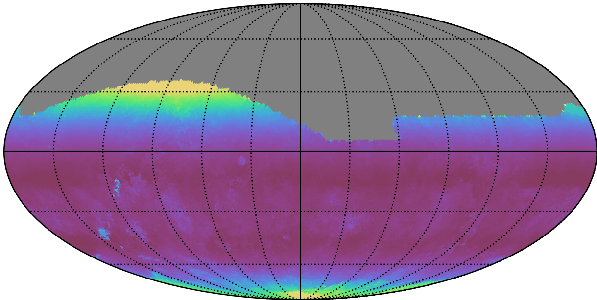
too_elab_r8_d2_gz_v3.4_10yrs All sky g band: Median airmass
