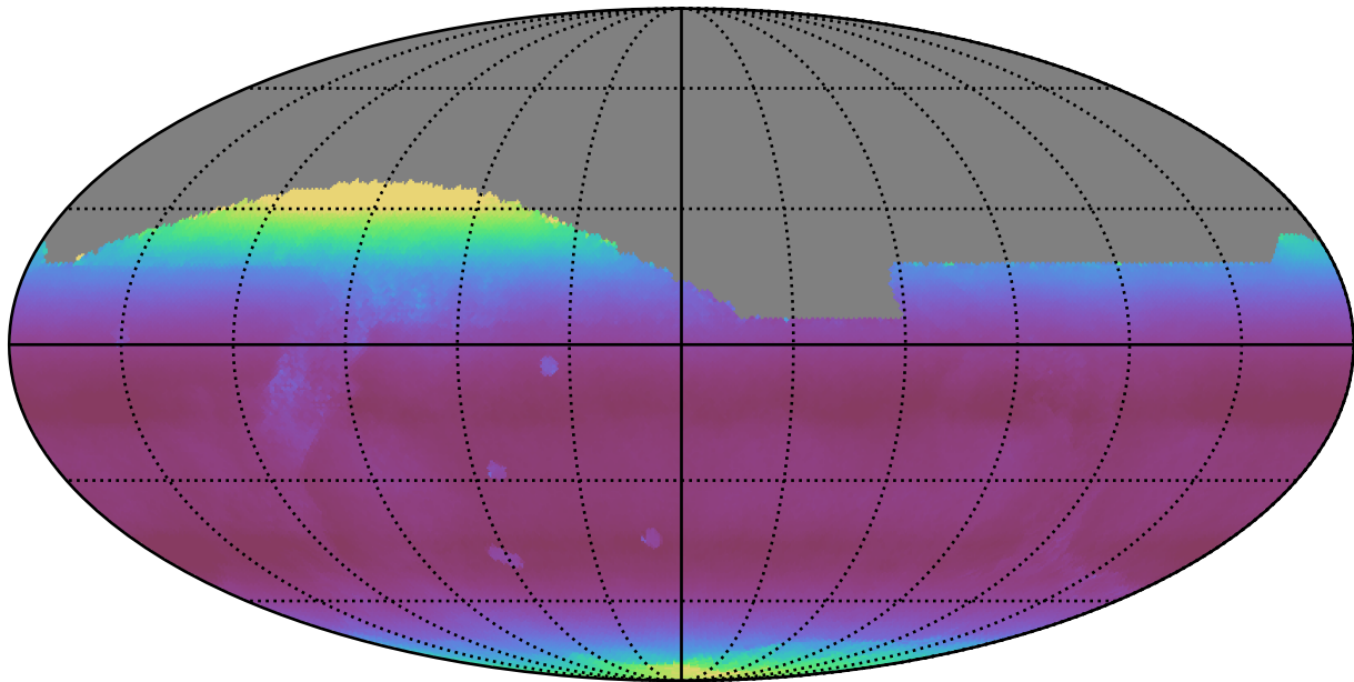
too_elab_r8_d2_gz_v3.4_10yrs All sky all bands: Median airmass
