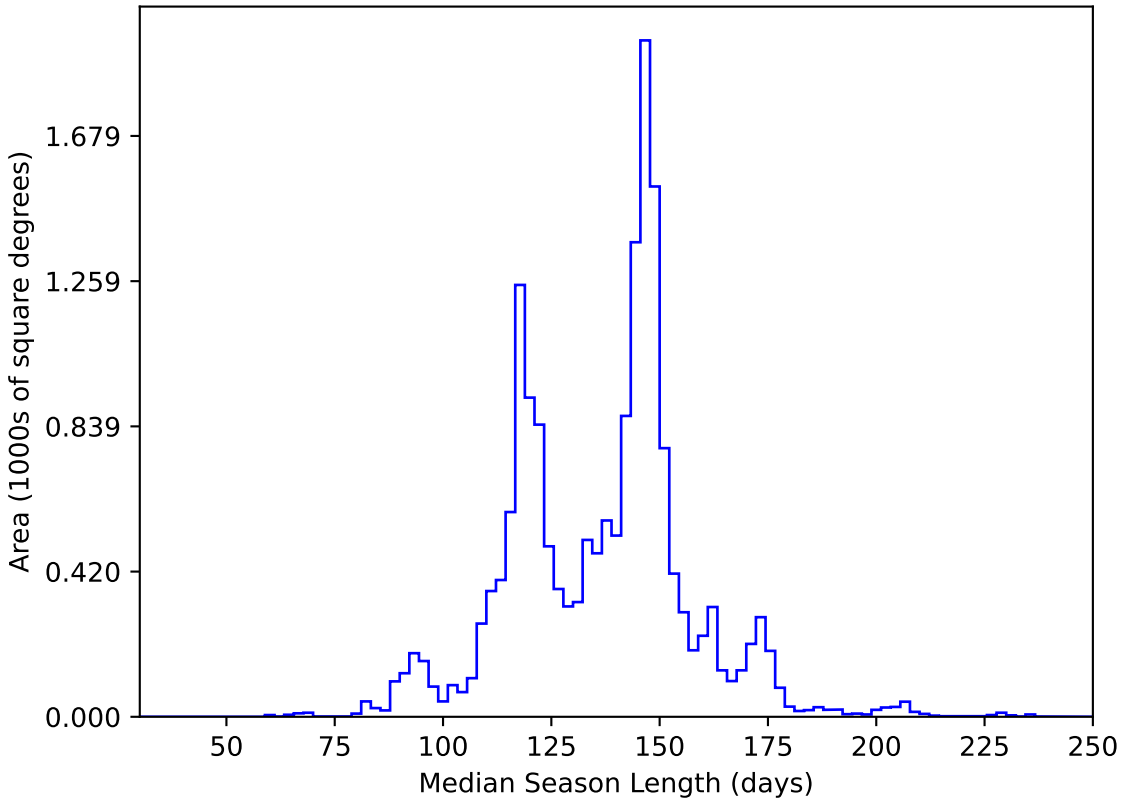
too_elab_r8_d2_gz_v3.4_10yrs WFD y band: Median Season Length
