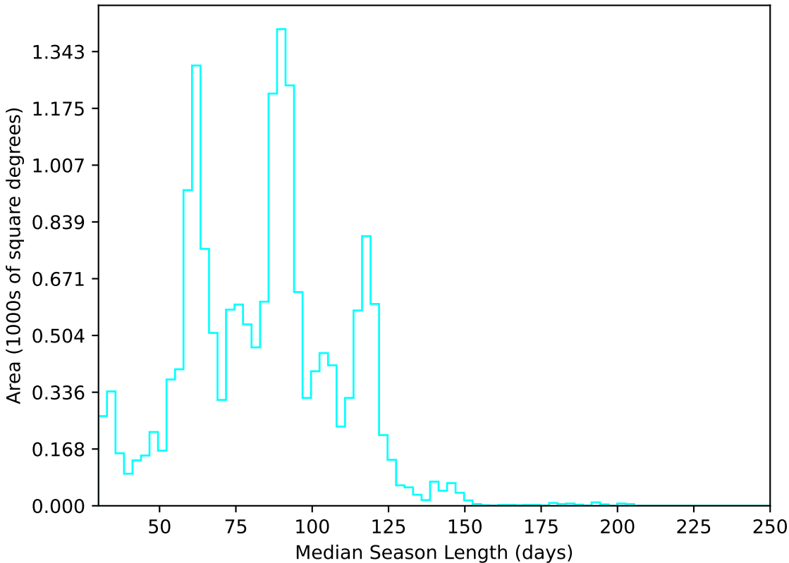
too_elab_r8_d2_gz_v3.4_10yrs WFD u band: Median Season Length
