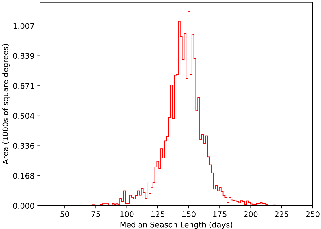
too_elab_r8_d2_gz_v3.4_10yrs WFD i band: Median Season Length
