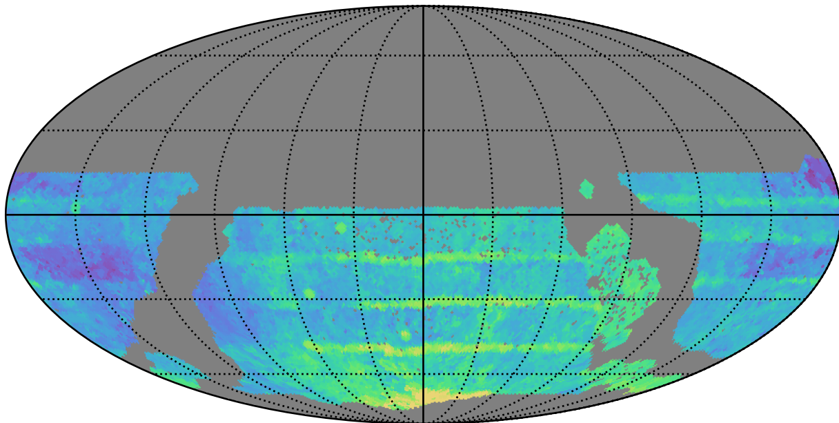
too_elab_r8_d2_gz_v3.4_10yrs WFD all bands: Median Season Length
