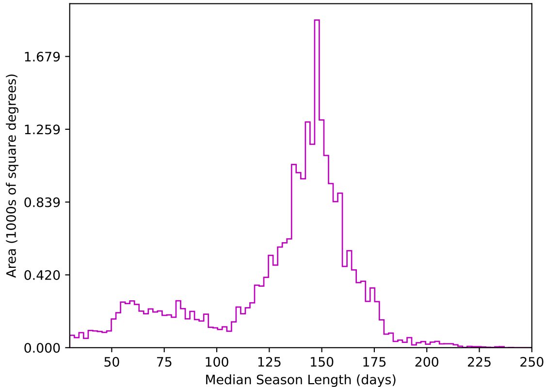
too_elab_r8_d2_gz_v3.4_10yrs All sky z band: Median Season Length
