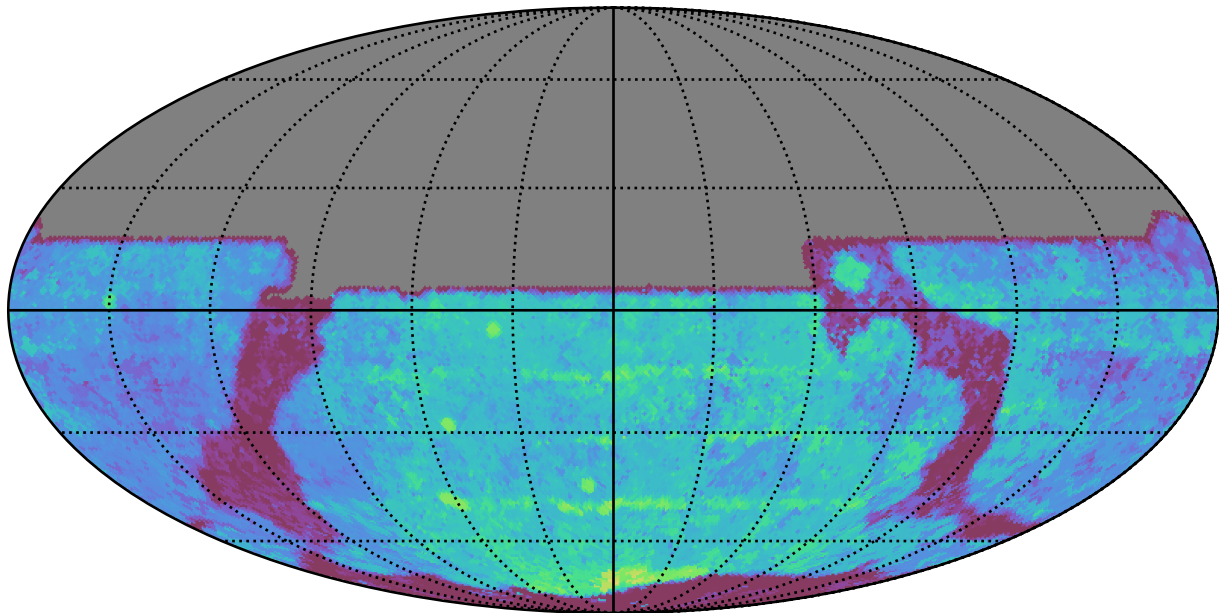
too_elab_r8_d2_gz_v3.4_10yrs All sky y band: Median Season Length
