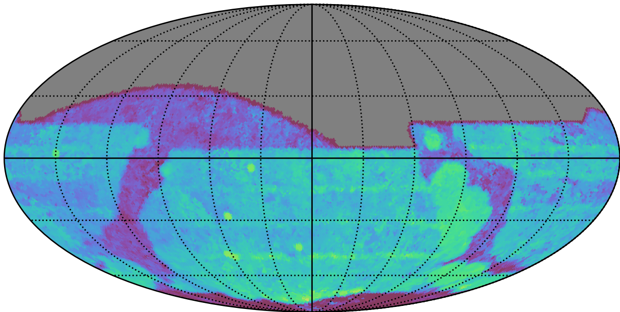
too_elab_r8_d2_gz_v3.4_10yrs All sky r band: Median Season Length
