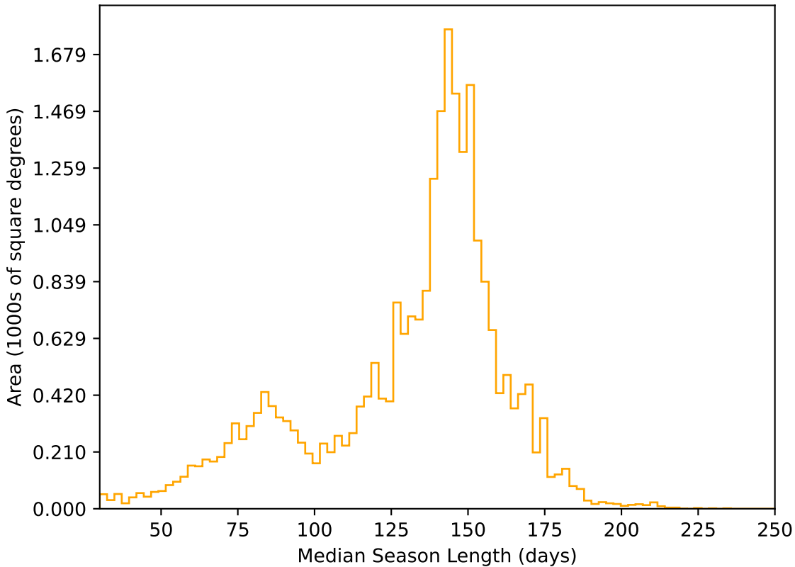
too_elab_r8_d2_gz_v3.4_10yrs All sky r band: Median Season Length
