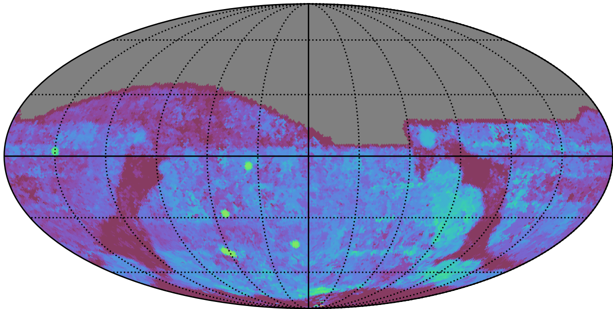
too_elab_r8_d2_gz_v3.4_10yrs All sky g band: Median Season Length
