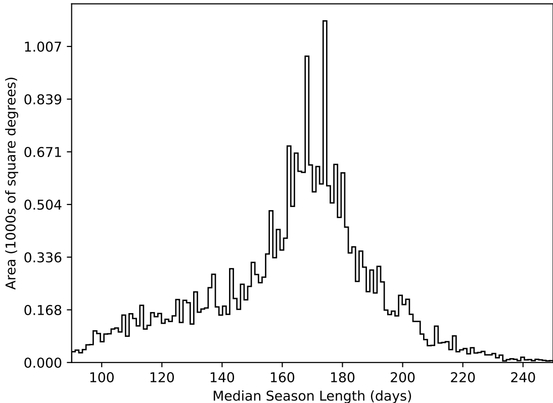
too_elab_r8_d2_gz_v3.4_10yrs All sky all bands: Median Season Length
