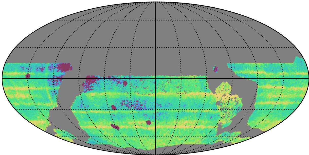
too_elab_r8_d2_gz_v3.4_10yrs WFD: Median Intra-Night Gap
