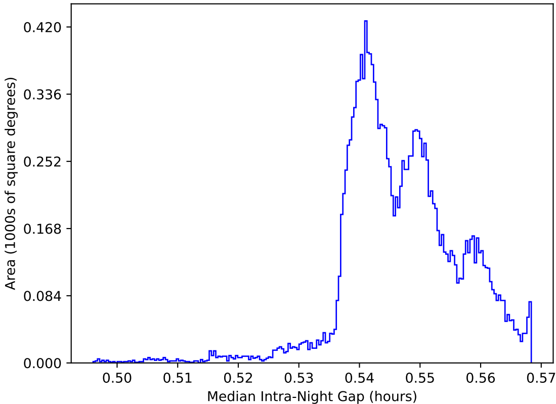
too_elab_r8_d2_gz_v3.4_10yrs WFD: Median Intra-Night Gap
