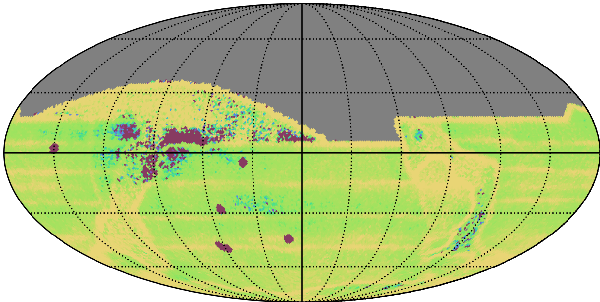
too_elab_r8_d2_gz_v3.4_10yrs All sky: Median Intra-Night Gap
