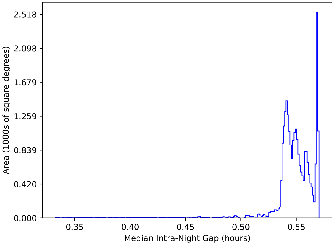
too_elab_r8_d2_gz_v3.4_10yrs All sky: Median Intra-Night Gap
