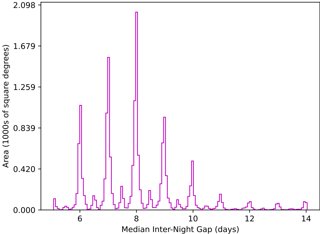
too_elab_r8_d2_gz_v3.4_10yrs WFD z band: Median Inter-Night Gap
