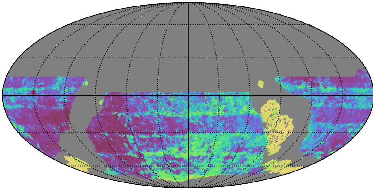
too_elab_r8_d2_gz_v3.4_10yrs WFD y band: Median Inter-Night Gap
