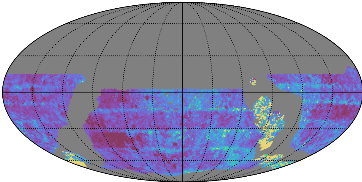
too_elab_r8_d2_gz_v3.4_10yrs WFD u band: Median Inter-Night Gap
