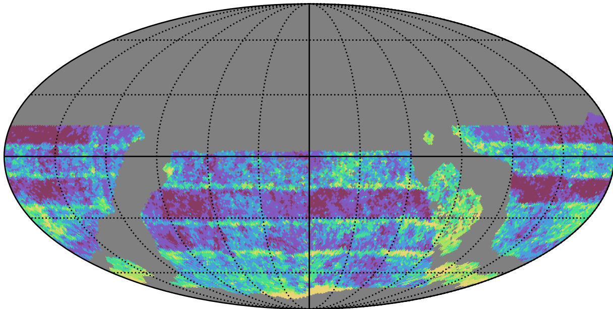
too_elab_r8_d2_gz_v3.4_10yrs WFD r band: Median Inter-Night Gap
