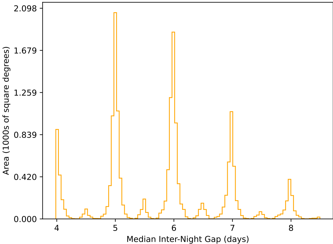
too_elab_r8_d2_gz_v3.4_10yrs WFD r band: Median Inter-Night Gap
