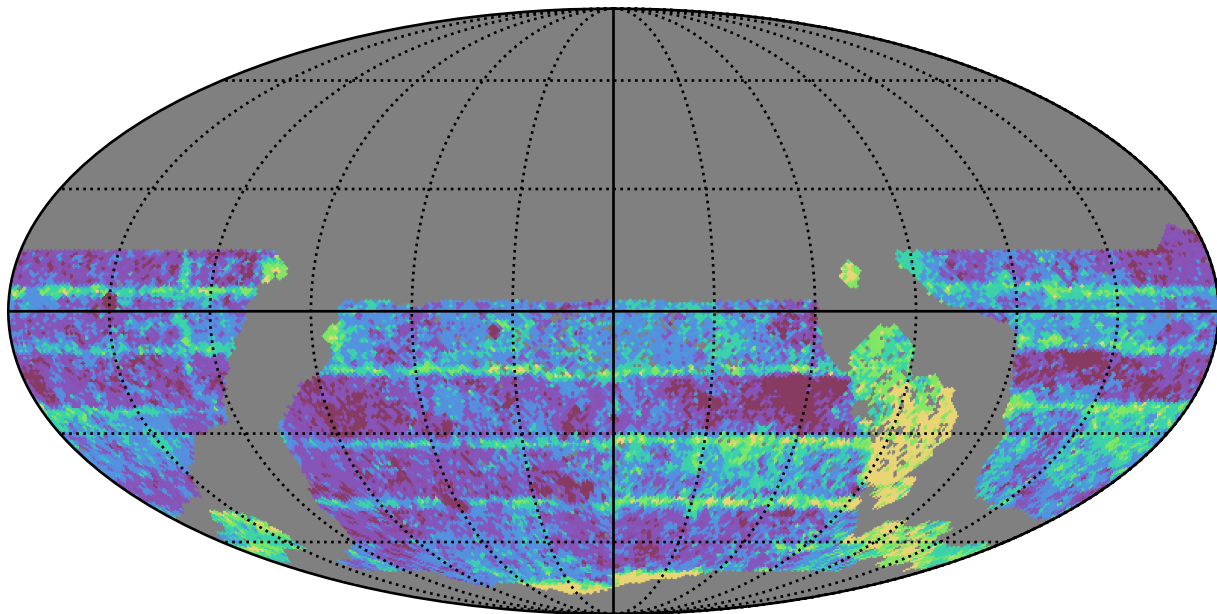
too_elab_r8_d2_gz_v3.4_10yrs WFD i band: Median Inter-Night Gap
