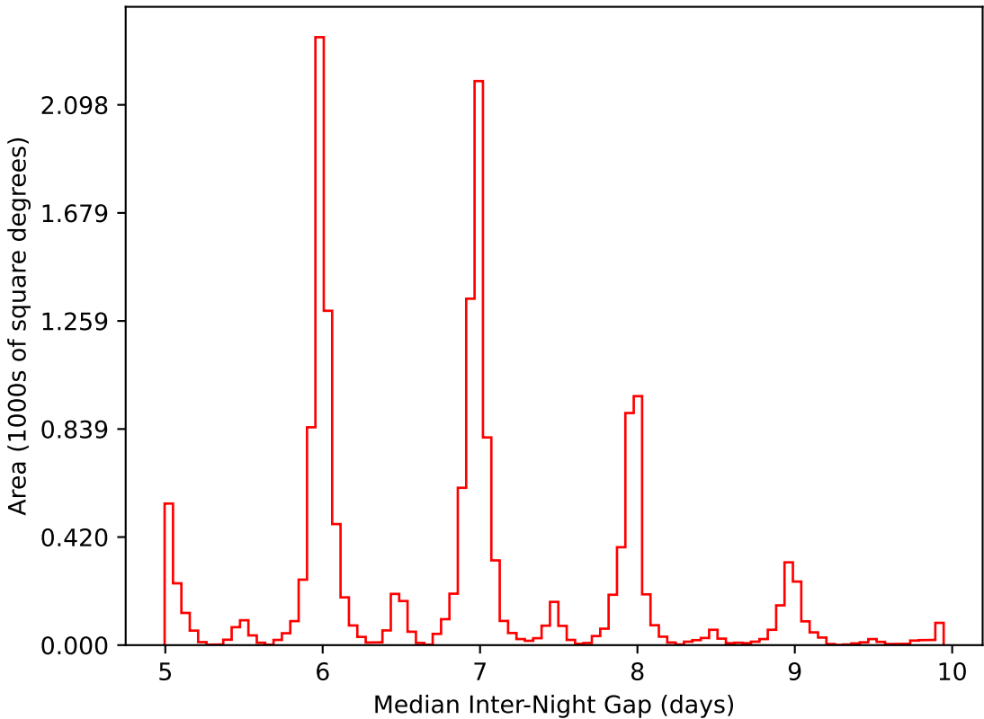
too_elab_r8_d2_gz_v3.4_10yrs WFD i band: Median Inter-Night Gap
