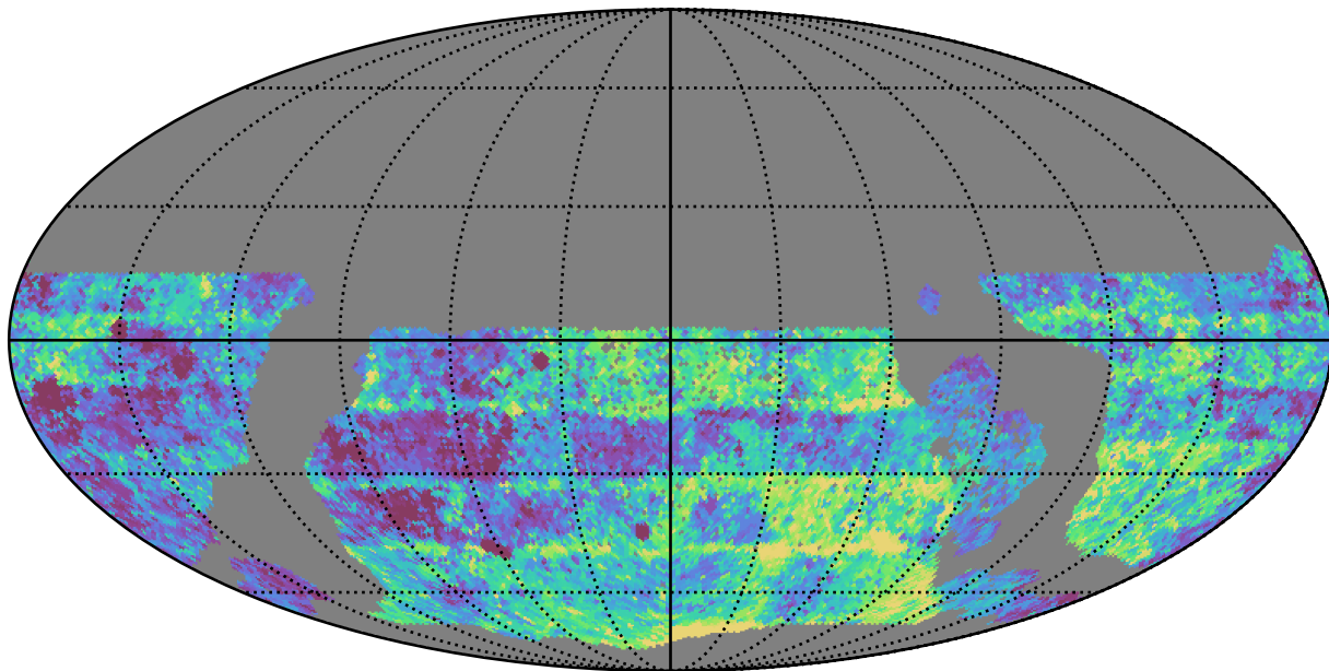
too_elab_r8_d2_gz_v3.4_10yrs WFD g band: Median Inter-Night Gap
