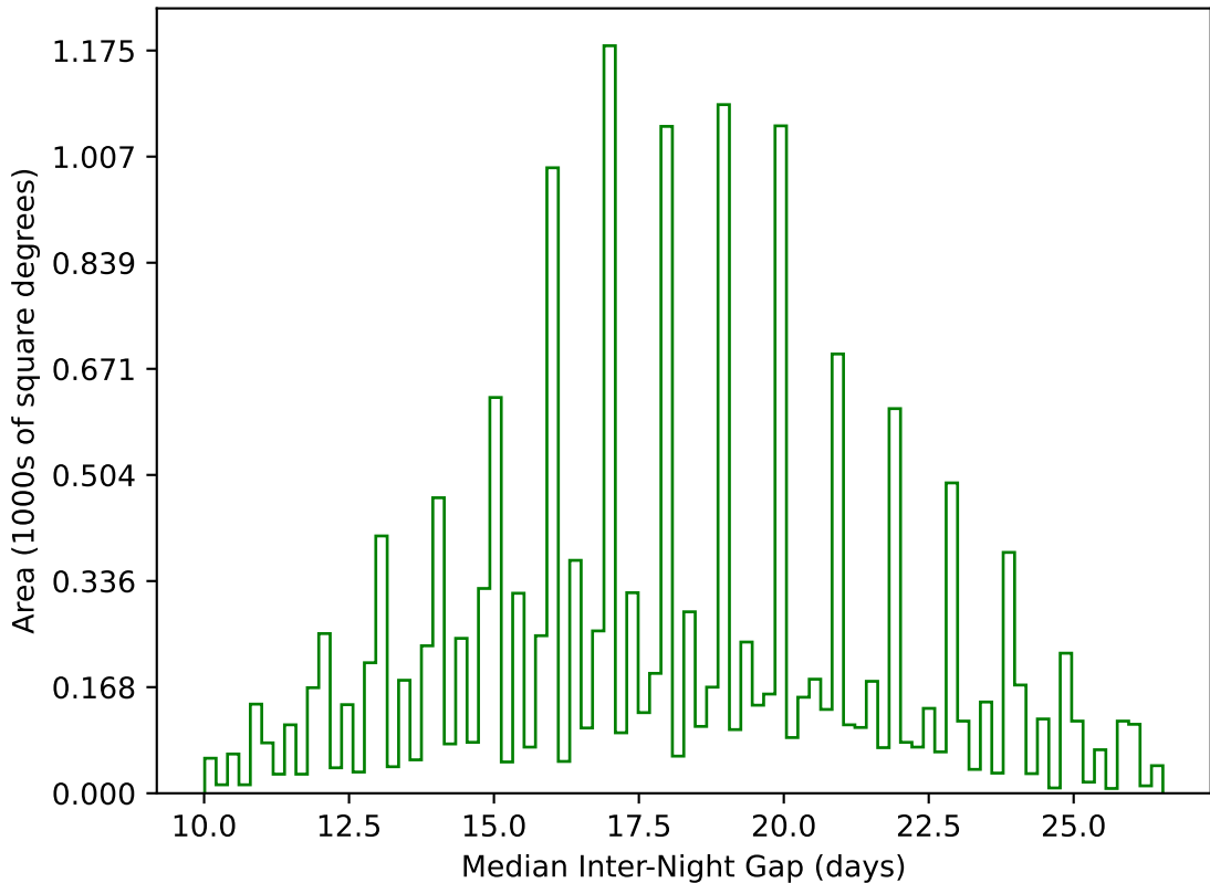
too_elab_r8_d2_gz_v3.4_10yrs WFD g band: Median Inter-Night Gap
