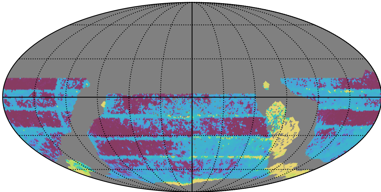
too_elab_r8_d2_gz_v3.4_10yrs WFD all bands: Median Inter-Night Gap
