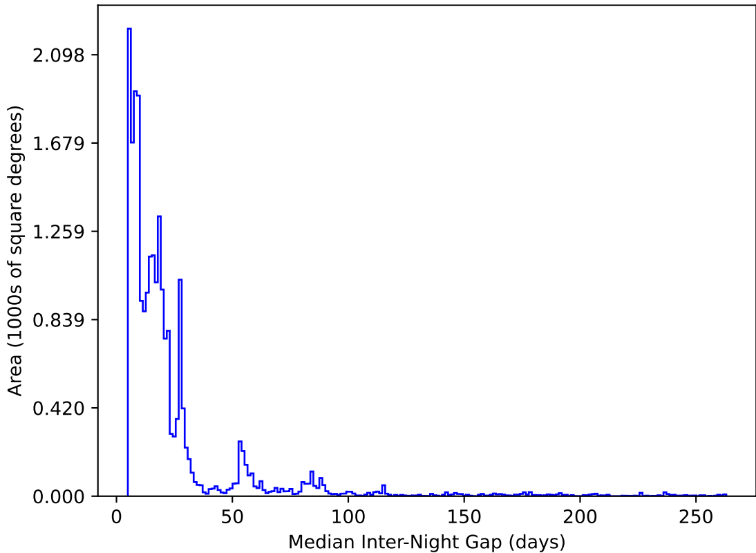
too_elab_r8_d2_gz_v3.4_10yrs All sky y band: Median Inter-Night Gap
