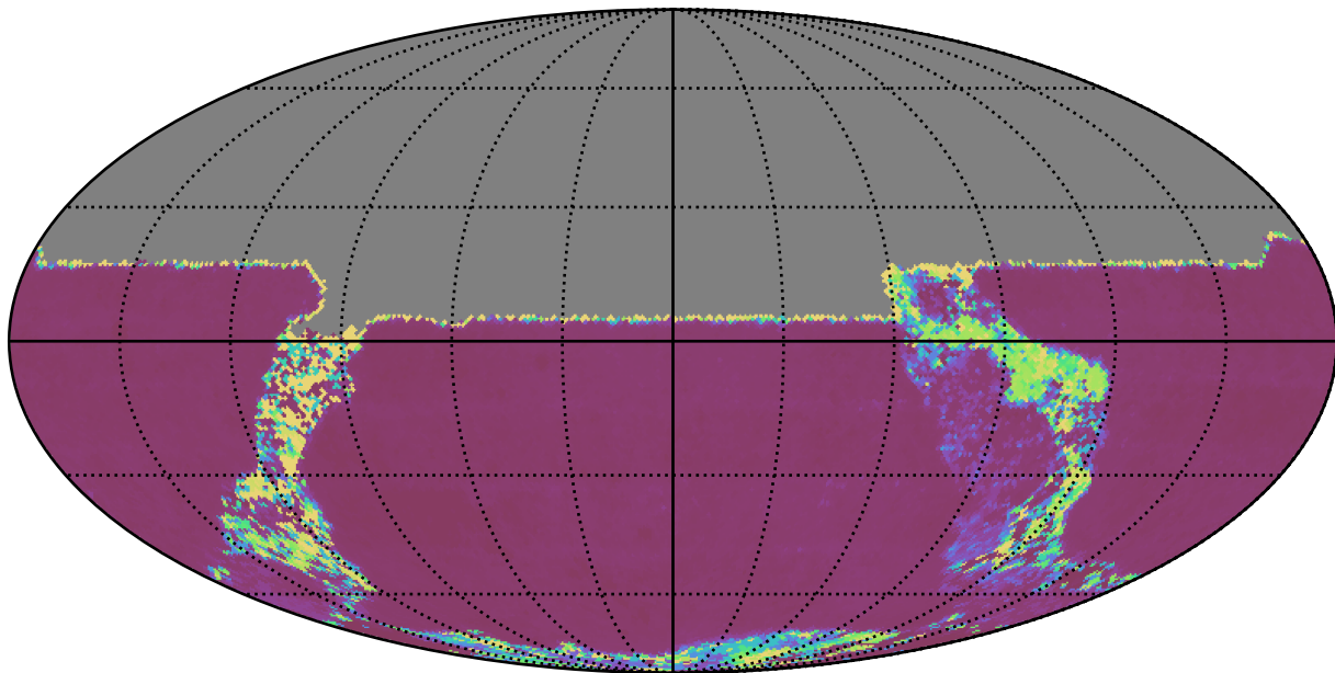
too_elab_r8_d2_gz_v3.4_10yrs All sky u band: Median Inter-Night Gap
