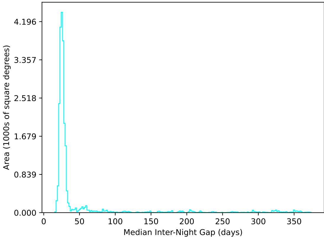
too_elab_r8_d2_gz_v3.4_10yrs All sky u band: Median Inter-Night Gap
