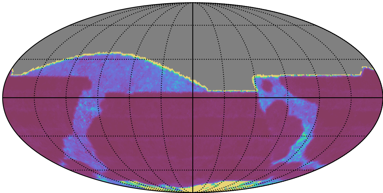
too_elab_r8_d2_gz_v3.4_10yrs All sky r band: Median Inter-Night Gap
