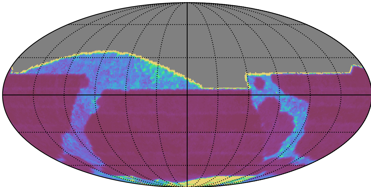
too_elab_r8_d2_gz_v3.4_10yrs All sky i band: Median Inter-Night Gap
