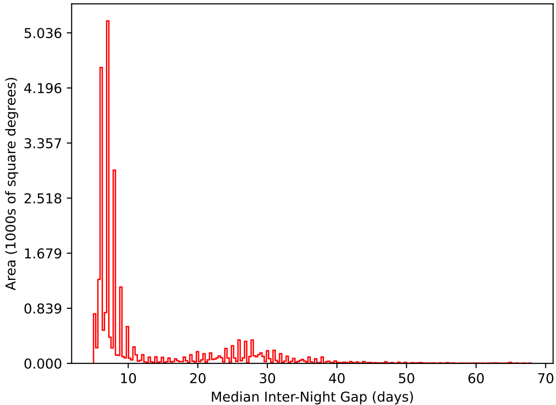
too_elab_r8_d2_gz_v3.4_10yrs All sky i band: Median Inter-Night Gap
