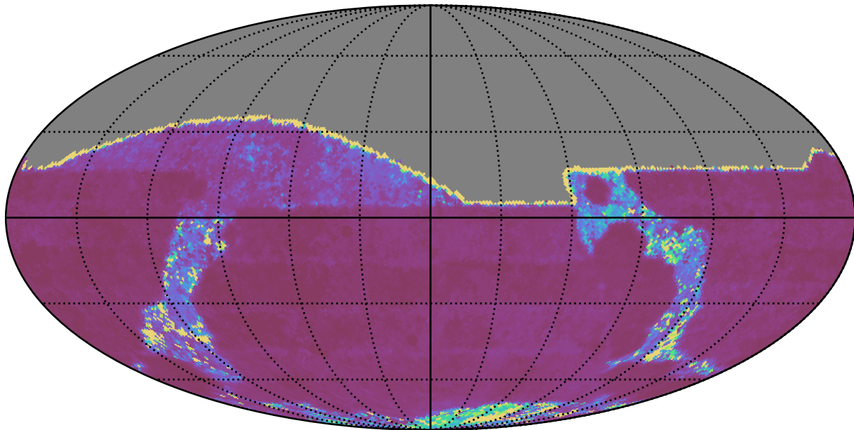
too_elab_r8_d2_gz_v3.4_10yrs All sky g band: Median Inter-Night Gap
