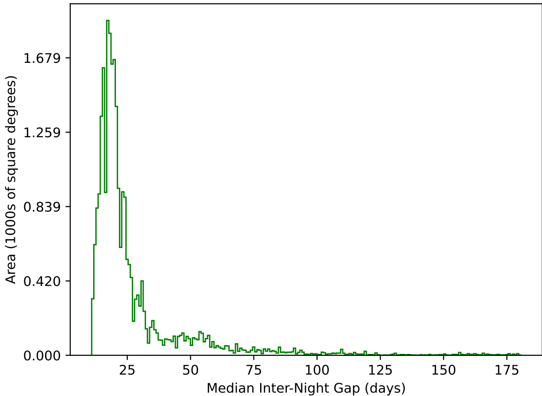
too_elab_r8_d2_gz_v3.4_10yrs All sky g band: Median Inter-Night Gap
