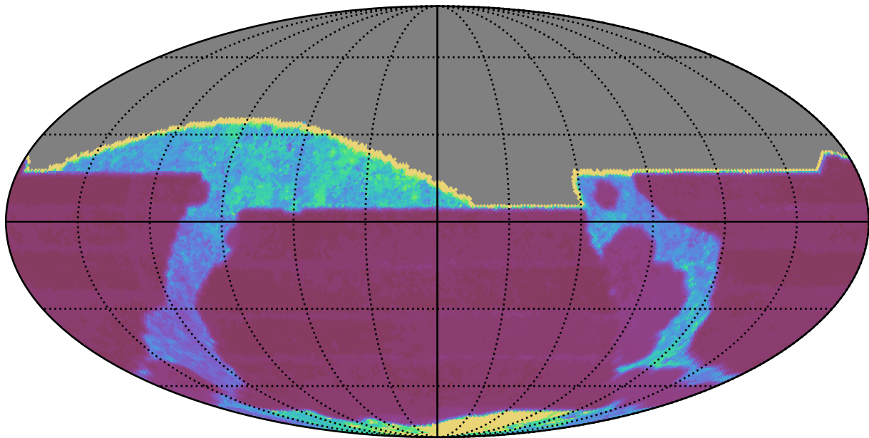
too_elab_r8_d2_gz_v3.4_10yrs All sky all bands: Median Inter-Night Gap
