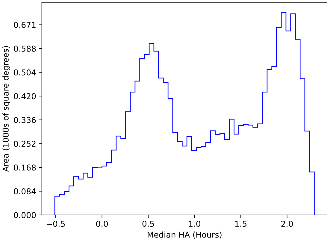
too_elab_r8_d2_gz_v3.4_10yrs WFD z band: Median HA
