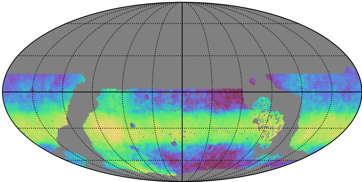
too_elab_r8_d2_gz_v3.4_10yrs WFD y band: Median HA
