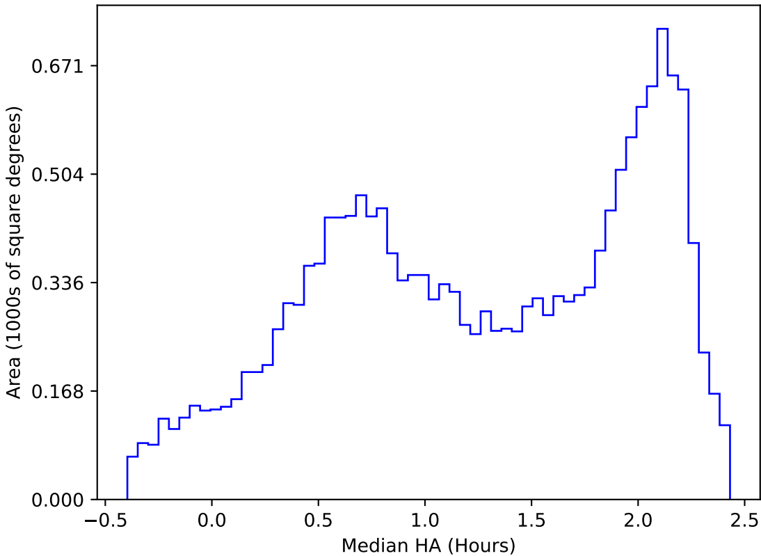
too_elab_r8_d2_gz_v3.4_10yrs WFD y band: Median HA
