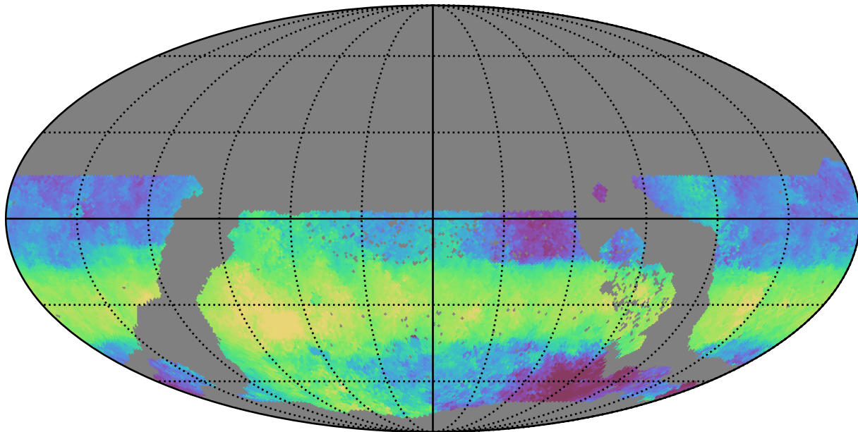
too_elab_r8_d2_gz_v3.4_10yrs WFD u band: Median HA
