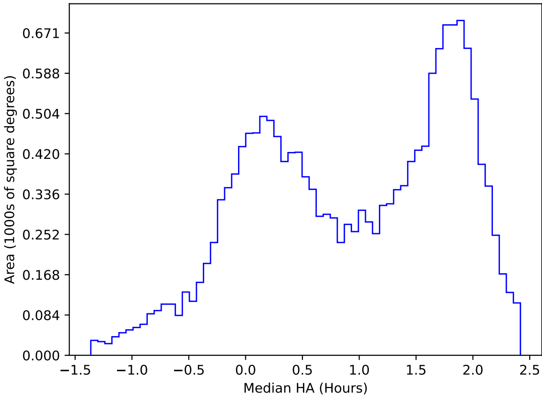
too_elab_r8_d2_gz_v3.4_10yrs WFD u band: Median HA
