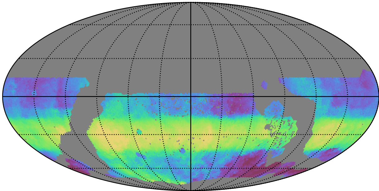
too_elab_r8_d2_gz_v3.4_10yrs WFD r band: Median HA
