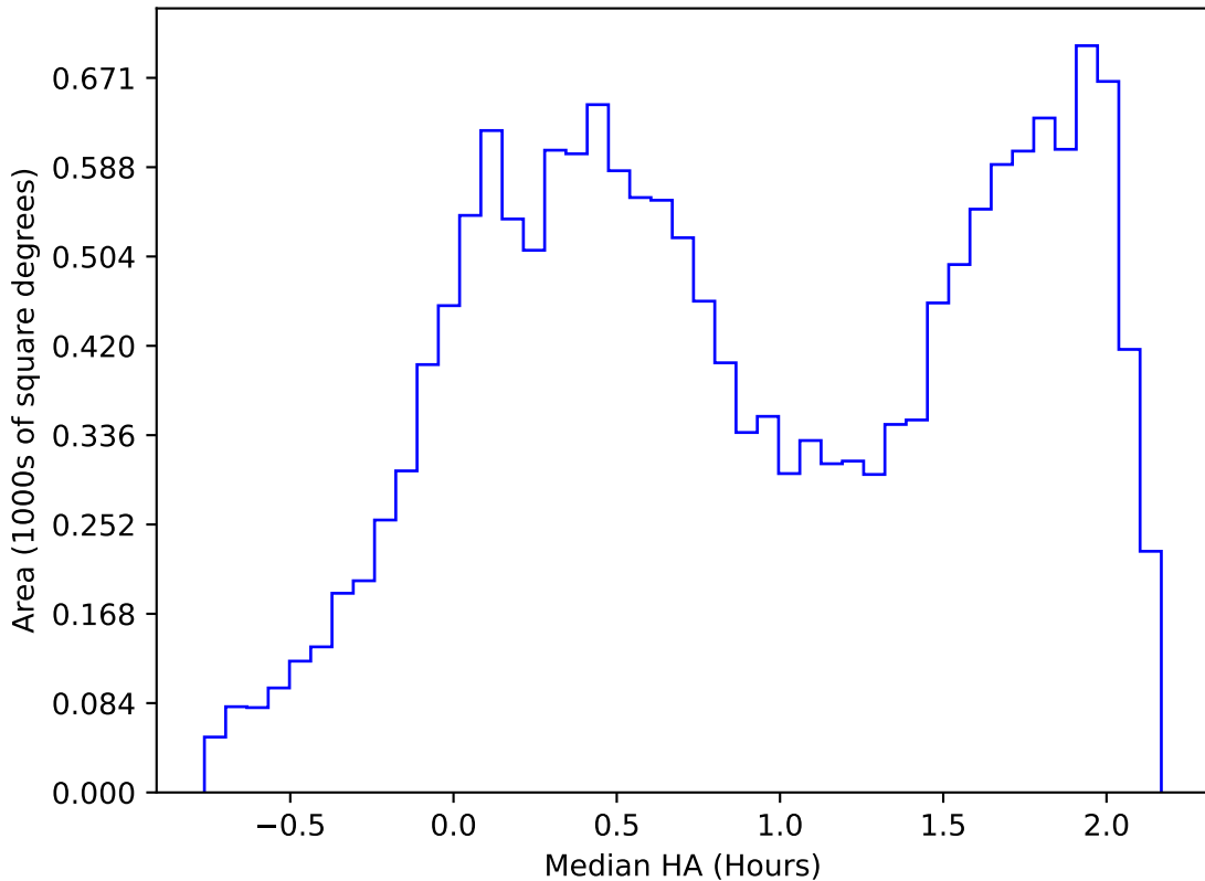
too_elab_r8_d2_gz_v3.4_10yrs WFD r band: Median HA
