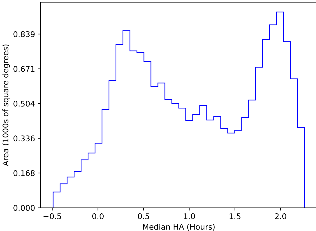
too_elab_r8_d2_gz_v3.4_10yrs WFD i band: Median HA
