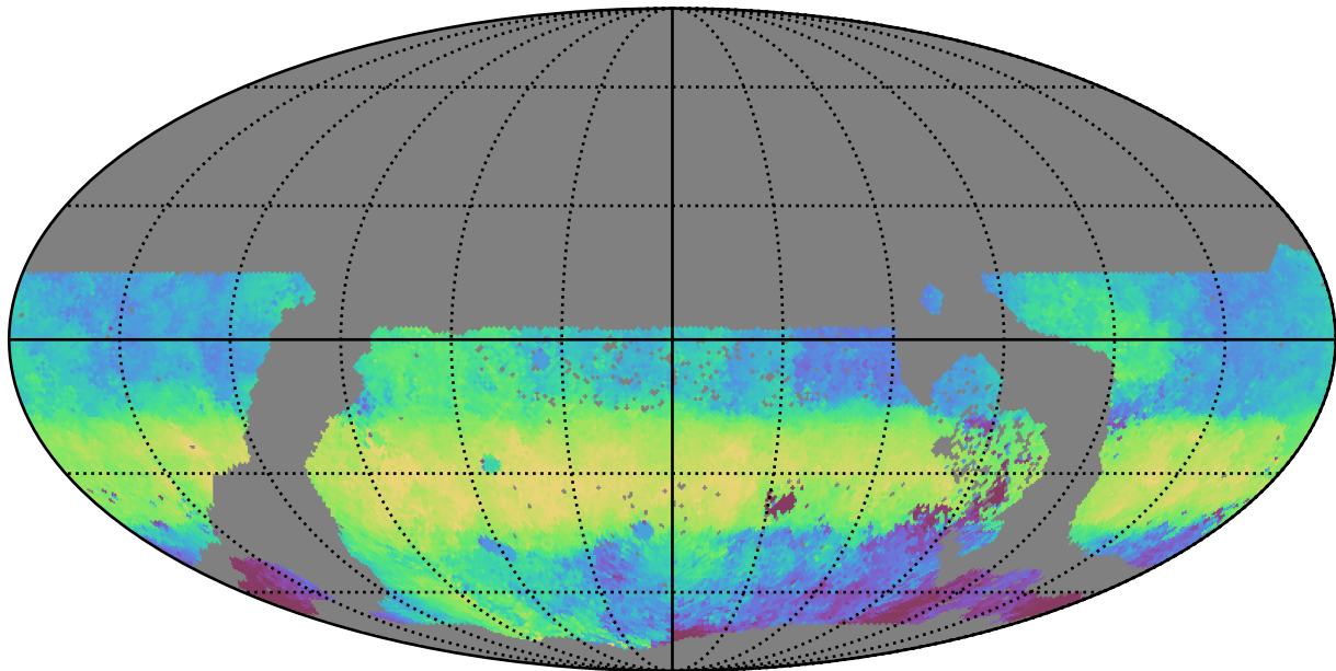
too_elab_r8_d2_gz_v3.4_10yrs WFD g band: Median HA
