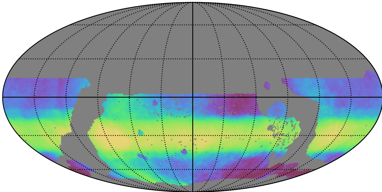
too_elab_r8_d2_gz_v3.4_10yrs WFD all bands: Median HA
