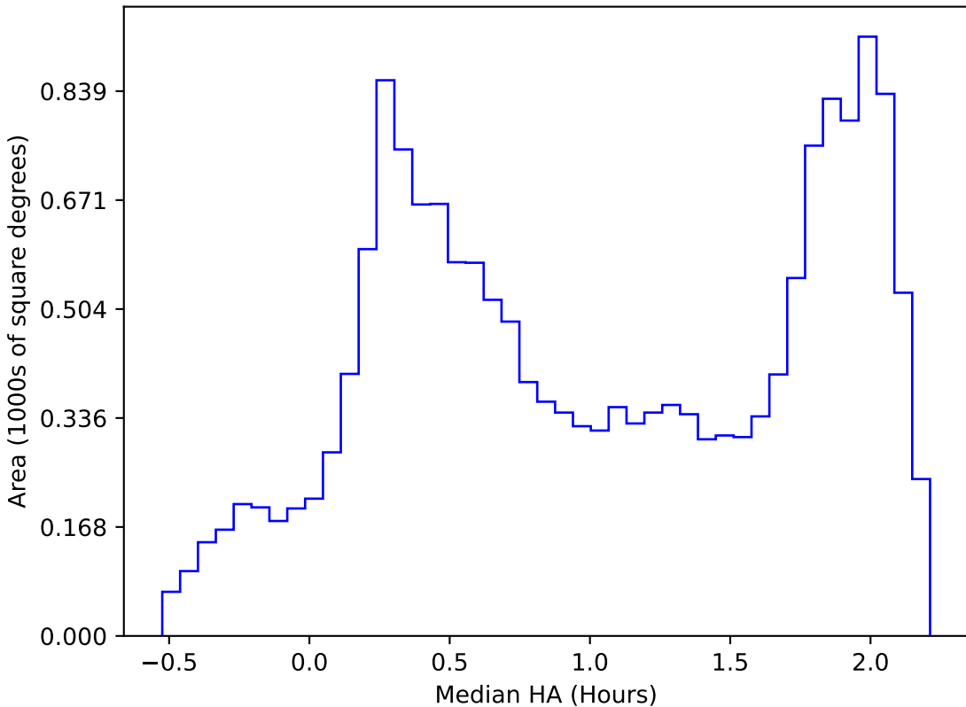
too_elab_r8_d2_gz_v3.4_10yrs WFD all bands: Median HA
