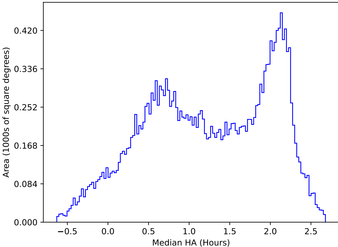
too_elab_r8_d2_gz_v3.4_10yrs All sky y band: Median HA
