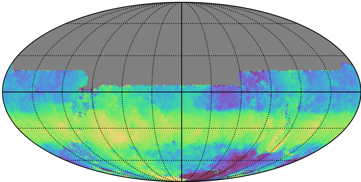
too_elab_r8_d2_gz_v3.4_10yrs All sky u band: Median HA
