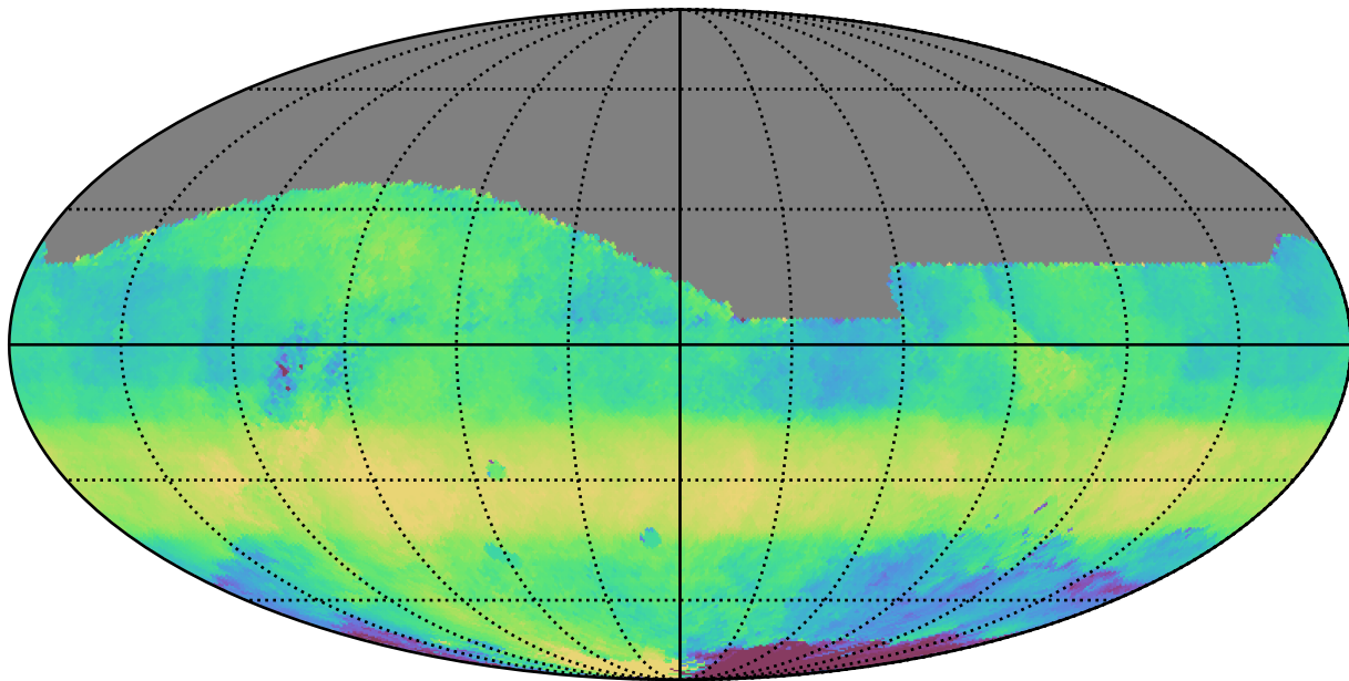
too_elab_r8_d2_gz_v3.4_10yrs All sky r band: Median HA
